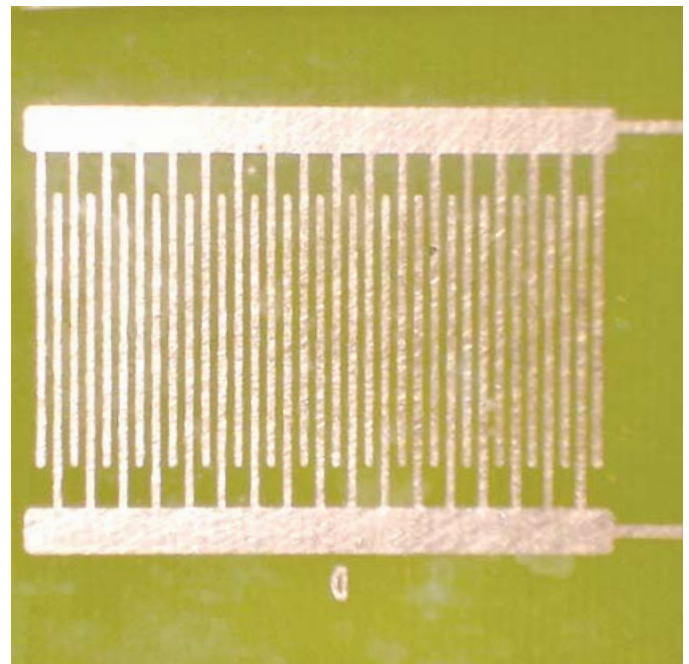
Close Up View of Submerged Comb – Note No Physical Contact Between Top and Bottom Combs
