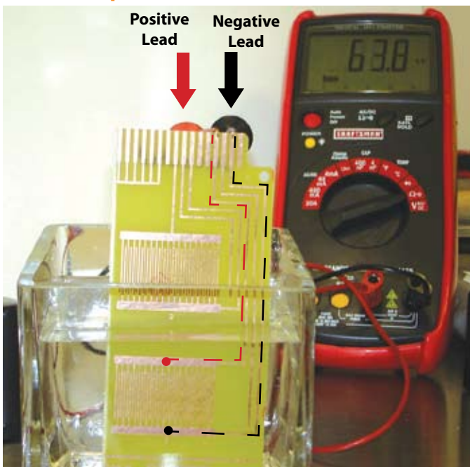
Test Set Up A – Submerged Comb Structure, Ohms vs Time
